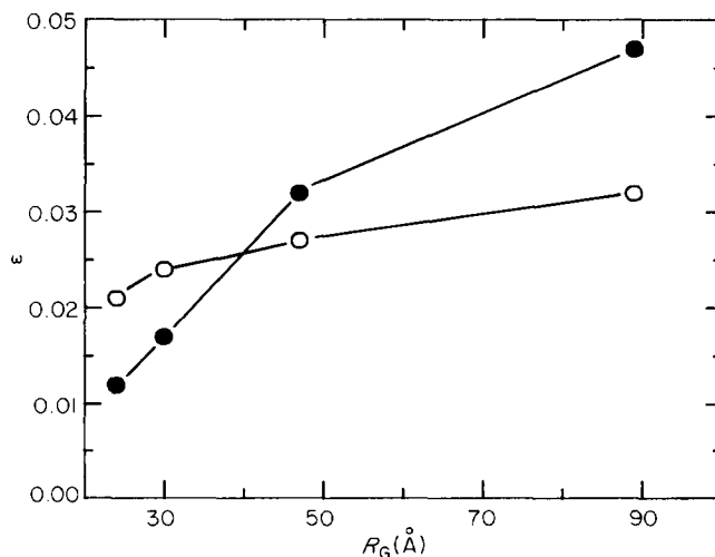
Figure 2 Equilibrium orientational coupling parameter, \varepsilon , measured at a constant stress of 0.84 MPa for low (○) and high (●) molecular weight PVE in PIP networks of varying crosslink density. The latter is connoted by the radius of gyration, R_G , calculated for the network strand length (Table 2). The R_G values for the PVE were 52 and 120 Å, respectively
